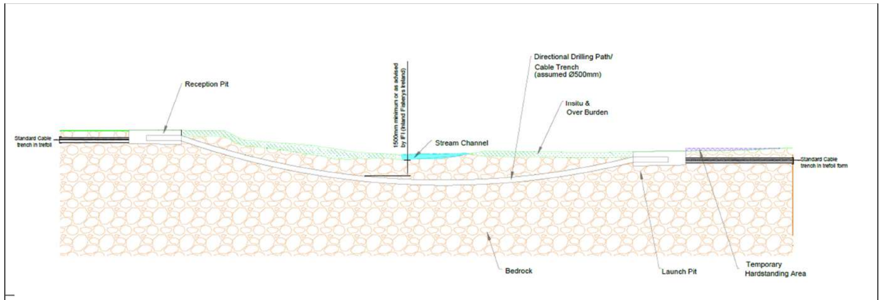
Figure 2-7 Typical Horizontal Directional Drill Water Crossing.
