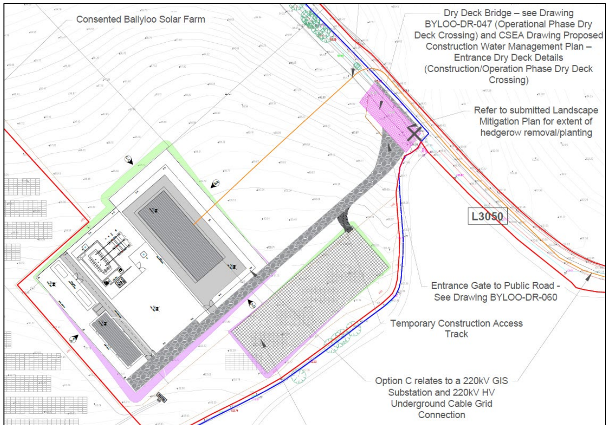
Figure 4: 220kV GIS Substation
