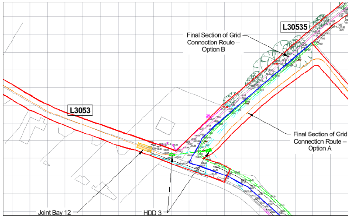
Figure 2-6 HDD between L-3053 & L-30535
