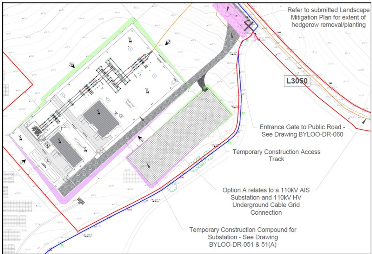
Figure 2: 110kV AIS Substation
