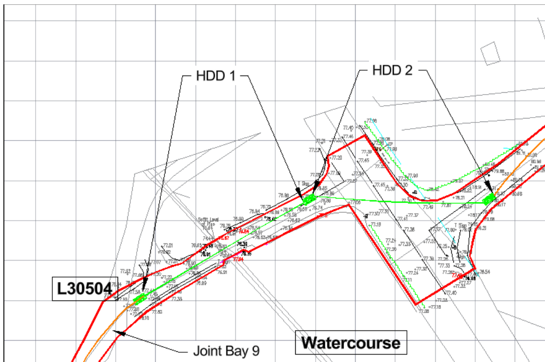
Figure 2-5 HDD under L30504 and N80
