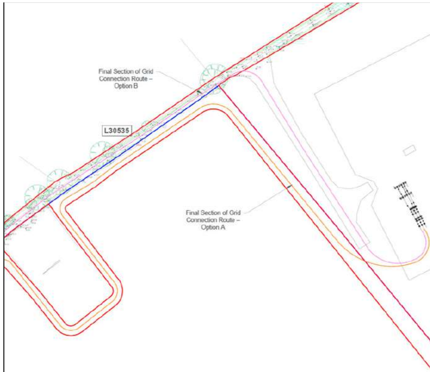
Figure 2-4 Alternative Grid Connection Routes into Existing Kellis Substation.
