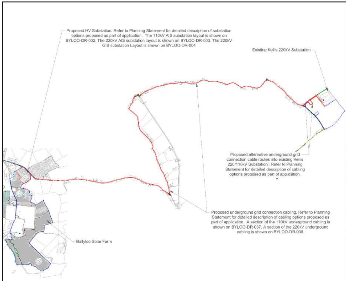
Figure 2.4 Underground Cabling Grid Connection Overview
