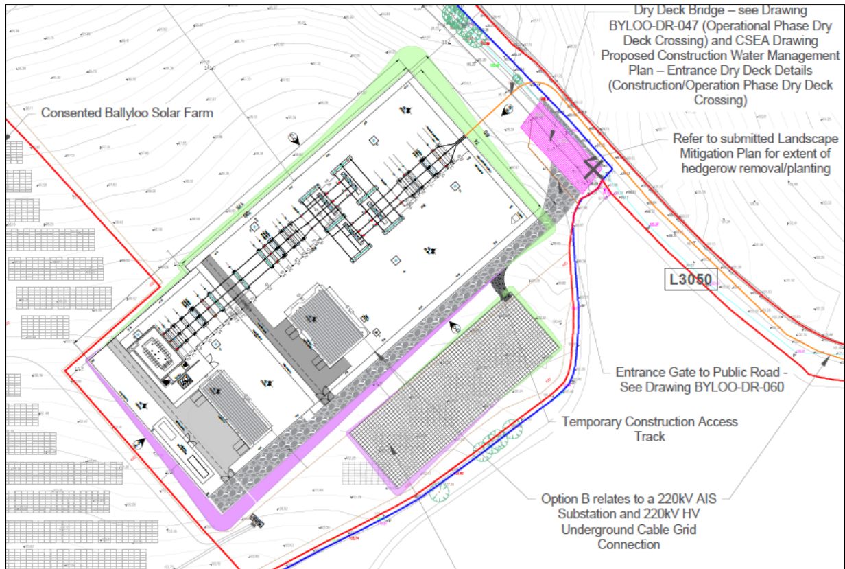
Figure 3: 220kV AIS Substation
